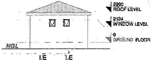
2 EAST ELEVATION 1:100
