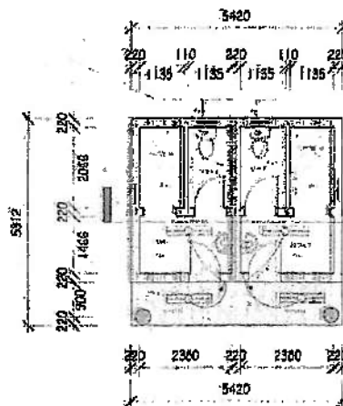
1 GROUND FLOOR 1:100
